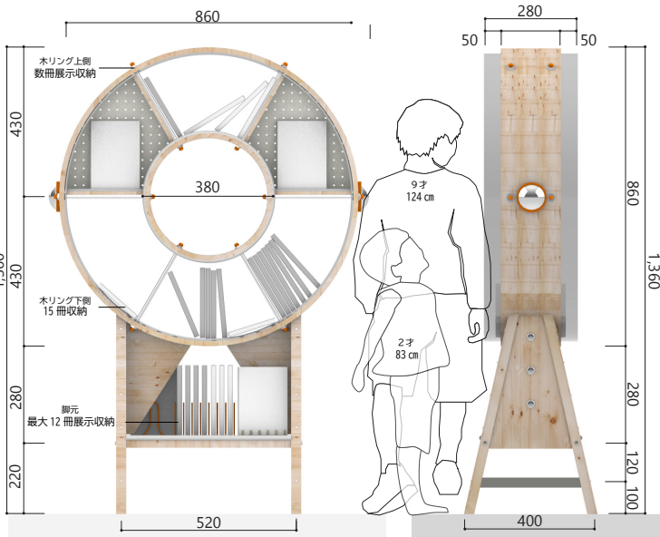
Front elevation (Scale:1/20) Side elevation (Scale:1/20)
